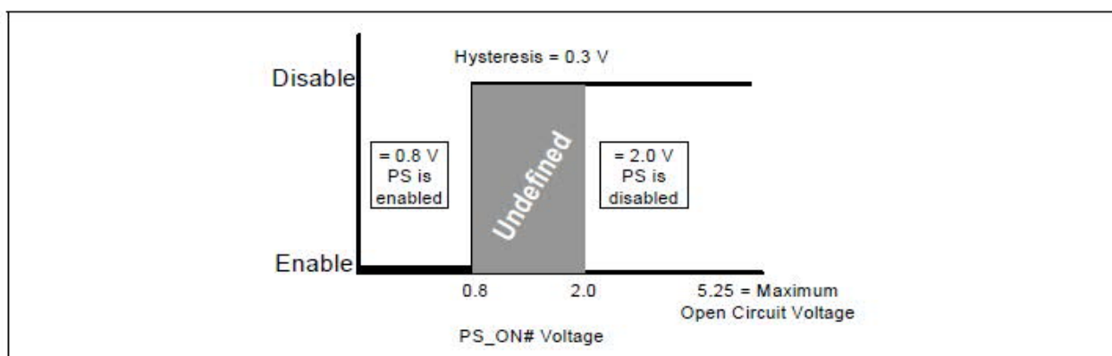
PS_ON# Signal Characteristics
