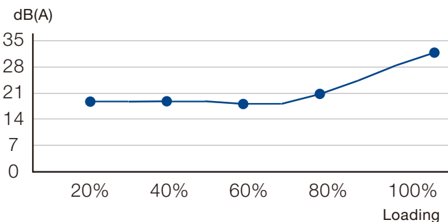
Acoustic Noise
