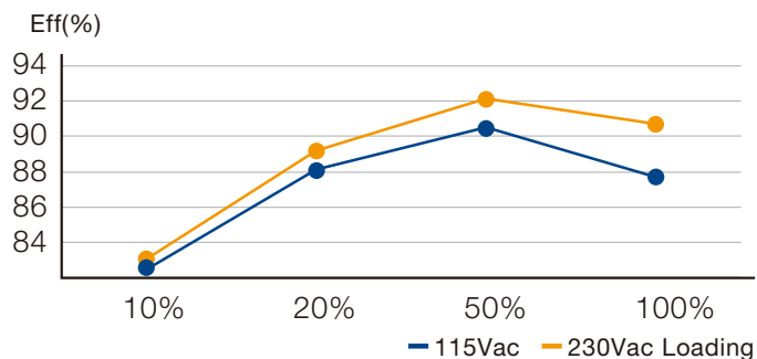
Efficiency
