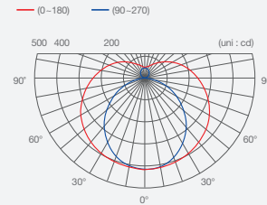
Light Distribution
