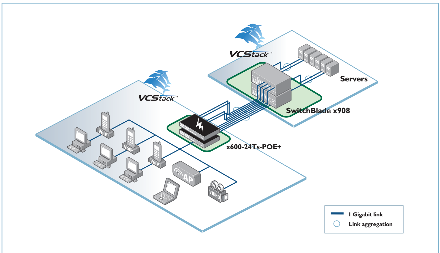
Diagram I: PoE+ Provision
