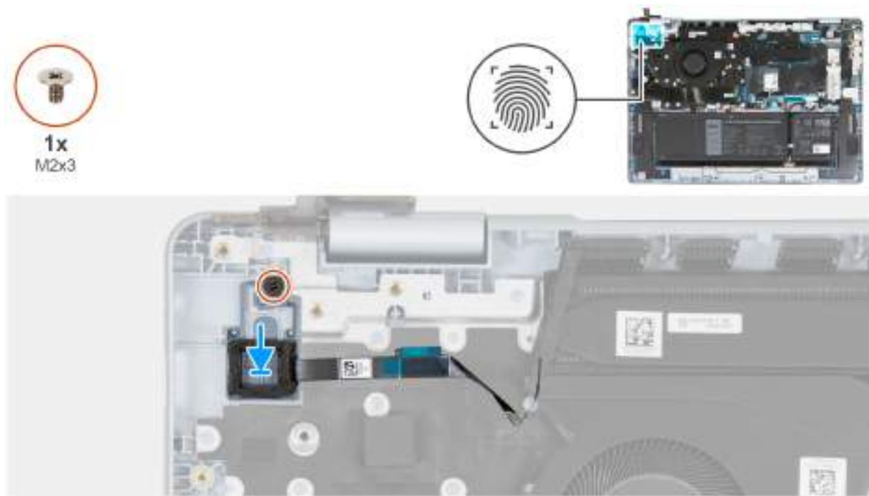
Figure 39. Installing power button with optional fingerprint reader
