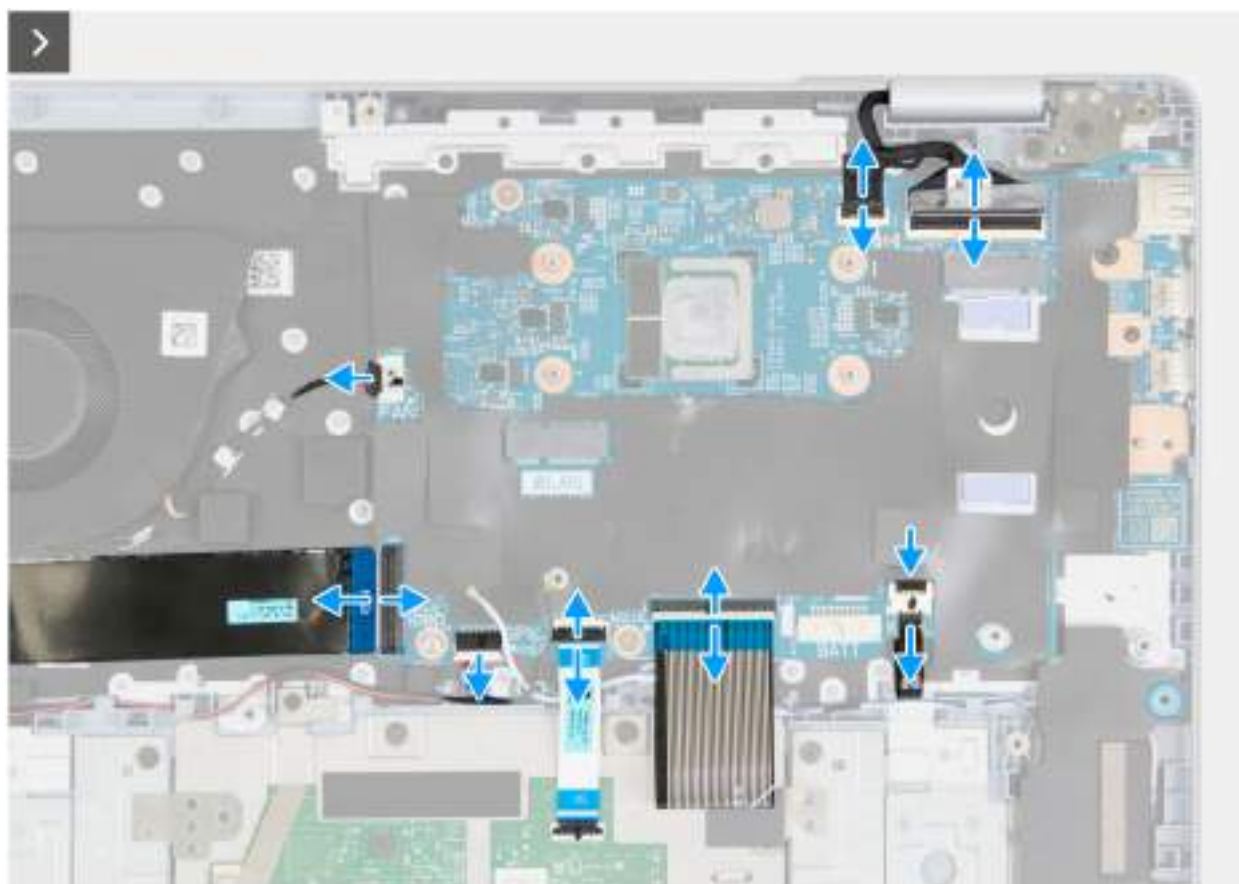
Figure 42. Removing the system board
