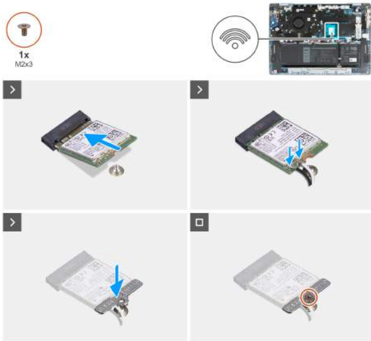
Figure 24. Installing the wireless card
