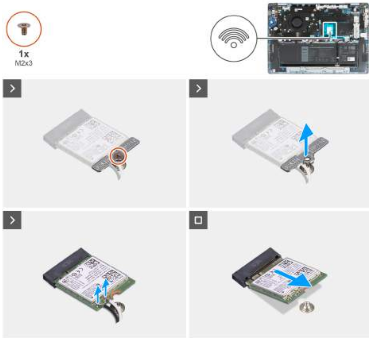
Figure 23. Removing the wireless card
