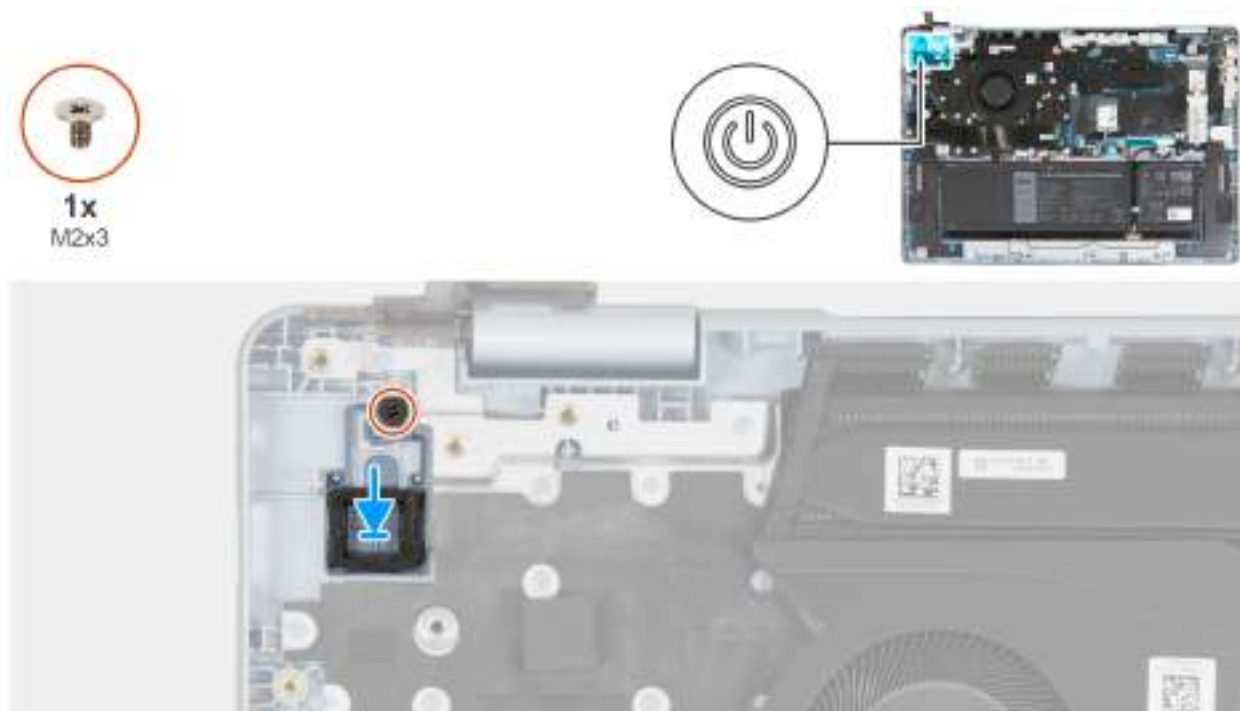
Figure 37. Installing power button
