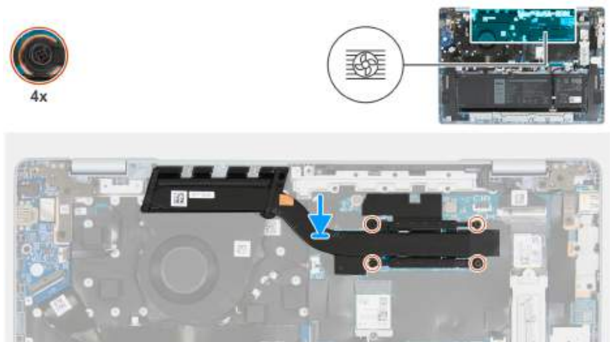
Figure 51. Installing the heat sink
