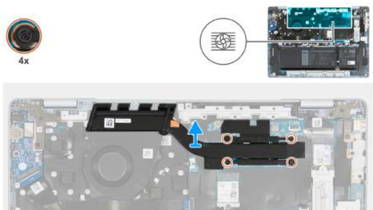
Figure 50. Removing the heat sink
