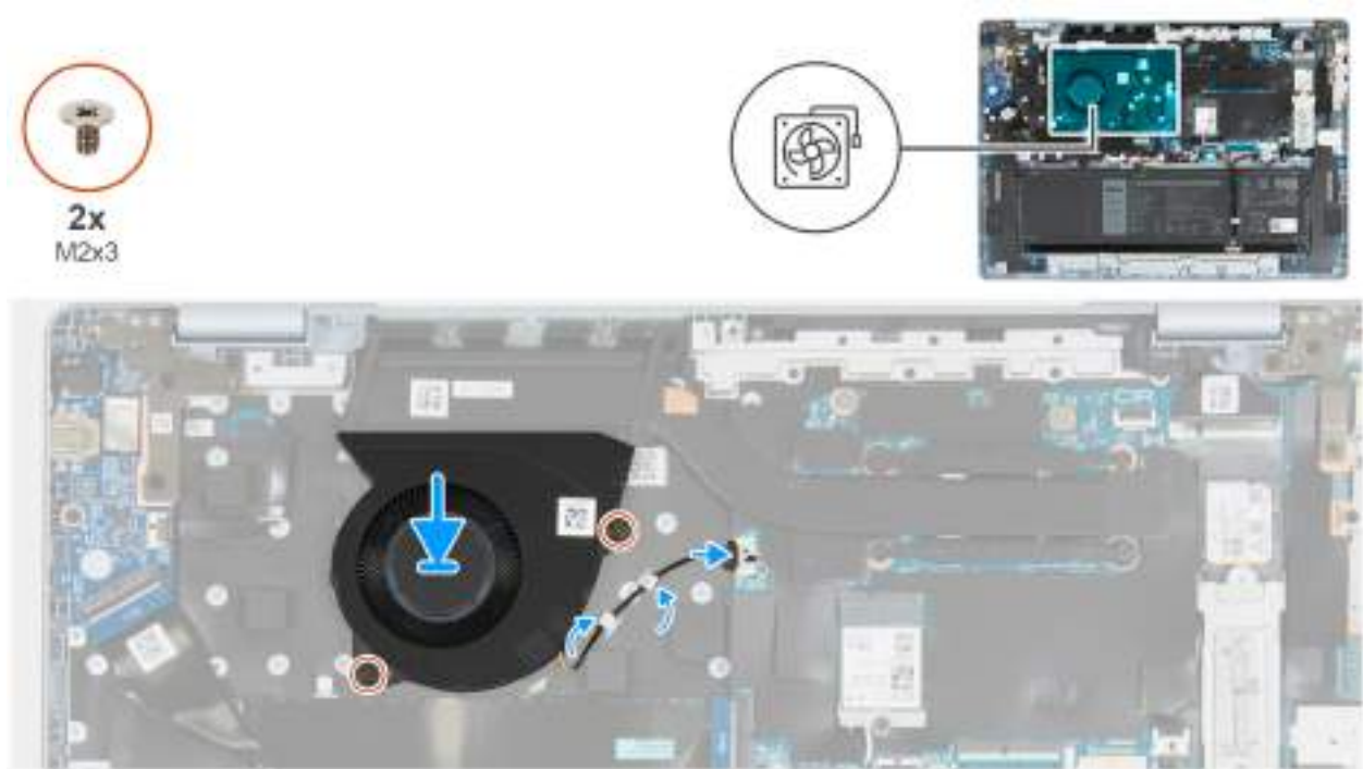
Figure 22. Installing the fan
