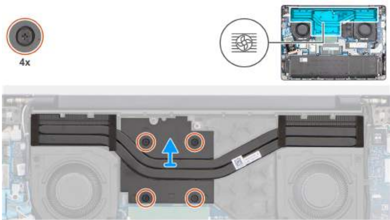
Figure 40. Removing the heat sink
