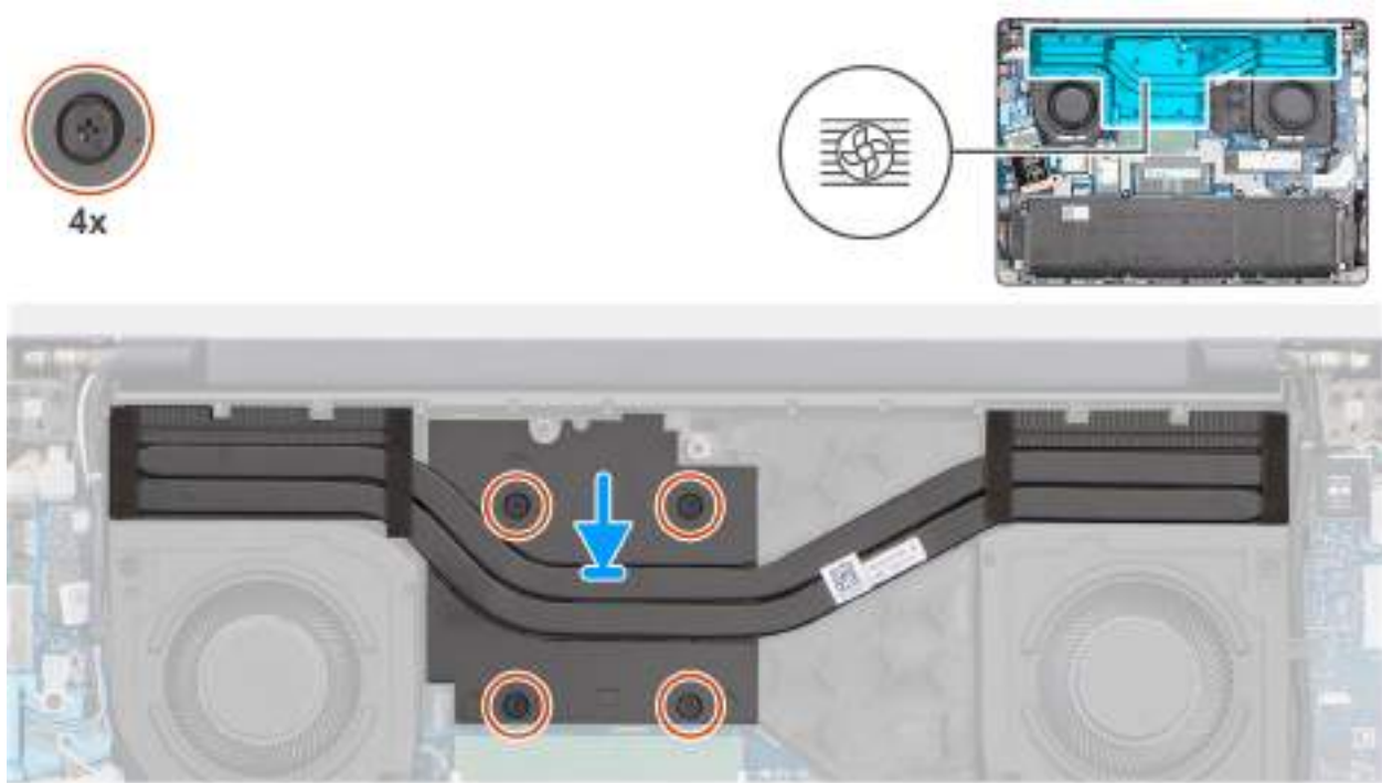
Figure 41. Installing the heat sink
