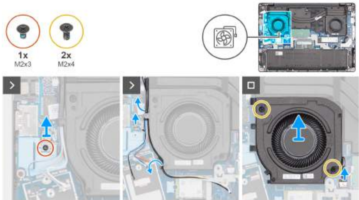
Figure 34. Removing the right/processor fan
