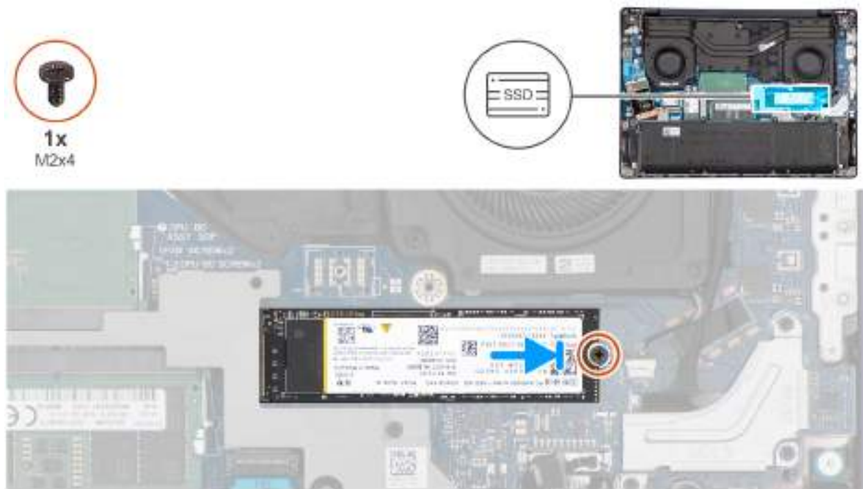
Figure 24. Installing the M.2 2280 solid state drive
