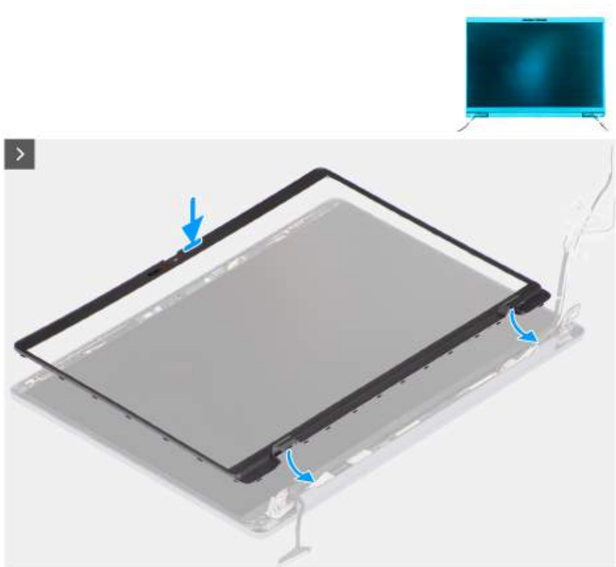
Figure 62. Installing the display bezel
