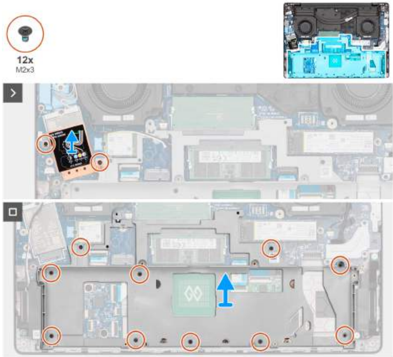
Figure 44. Removing the battery frame
