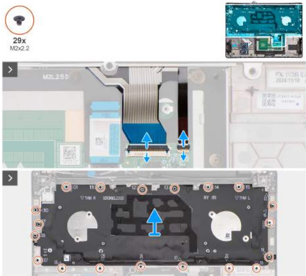
Figure 88. Removing the keyboard
